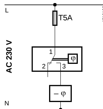
Diagram 2: Dehumidification
